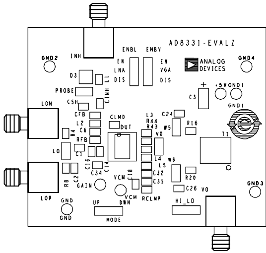
Figure 98. AD8331-EVALZ Assembly
