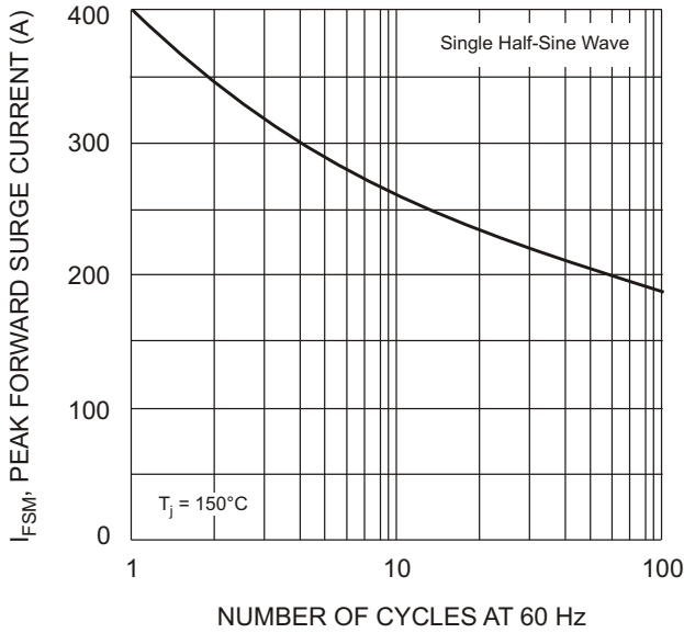
Fig. 3 Max Non-Repertive Surge Current
