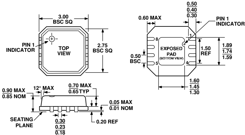
Figure 52. 8-Lead Lead Frame Chip Scale Package [LFCSP_VD]
