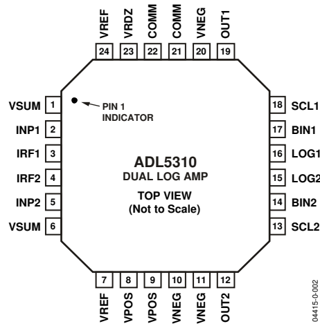
Figure 2. 24-Lead LFCSP Pin Configuration
