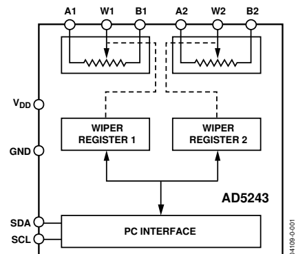
Figure 1. AD5243
