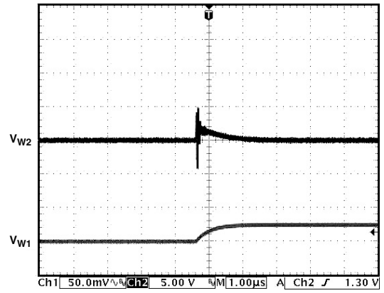
Figure 27. Analog Crosstalk
