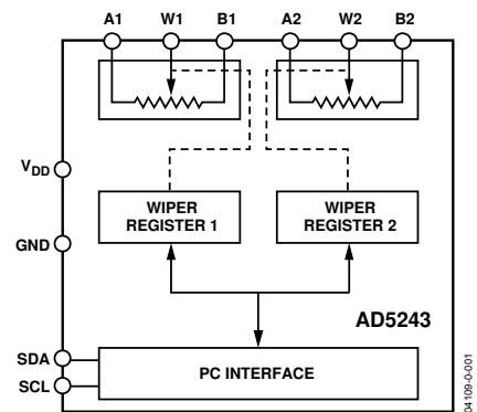
Figure 1. AD5243
