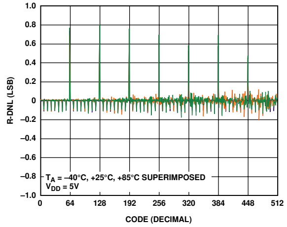
Figure 7. R-DNL—9-Bit RDAC
