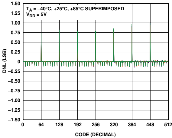
Figure 5. DNL—9-Bit RDAC
