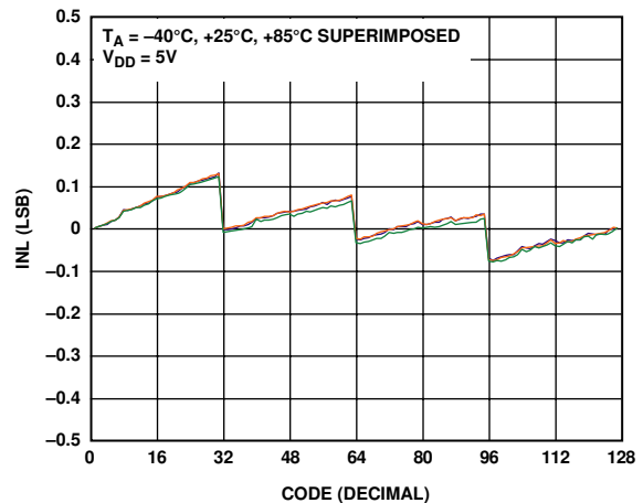
Figure 8. INL—7-Bit RDAC
