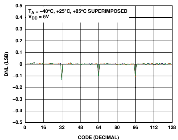
Figure 9. DNL—7-Bit RDAC
