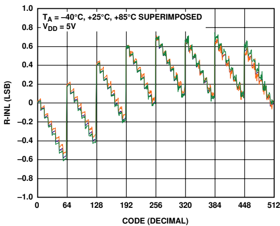
Figure 6. R-INL—9-Bit RDAC
