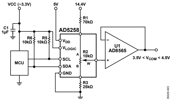
Figure 44. V_{COM} Adjustment Application
