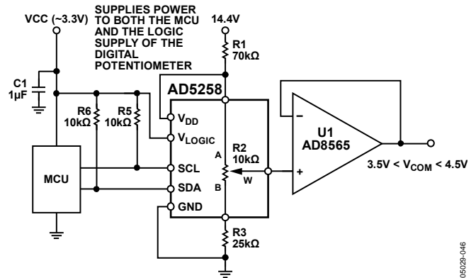
Figure 45. Circuitry When a Separate Supply Is Not Available for V_{DD}
