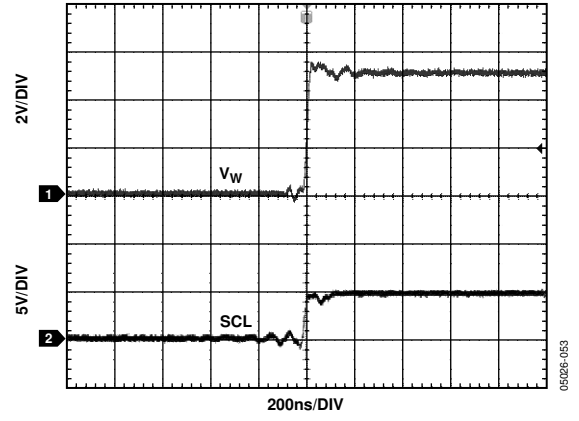
Figure 31. Large Signal Settling Time
