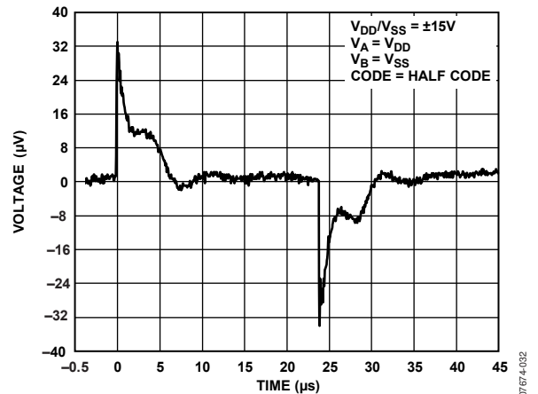
Figure 53. Digital Feedthrough
