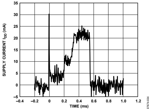
Figure 49. I_{DD} Waveform While Blowing/Reading Fuse
