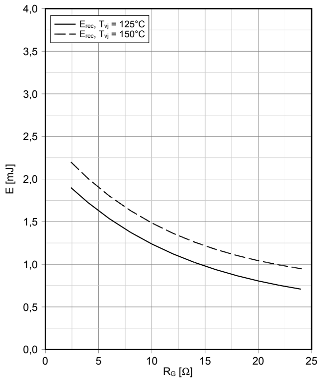
Schaltverluste Diode, 3-Level (typisch) switching losses Diode, 3-Level (typical) E_{rec} = f(R_G) I_F = 150 A, V_{CE} = 350 V
