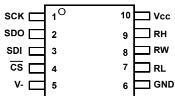
ISL22414 (10 LD MSOP) TOP VIEW
