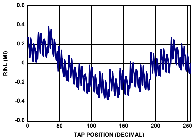
FIGURE 9. 10k RINL vs TAP POSITION, V_{CC} = 5V
