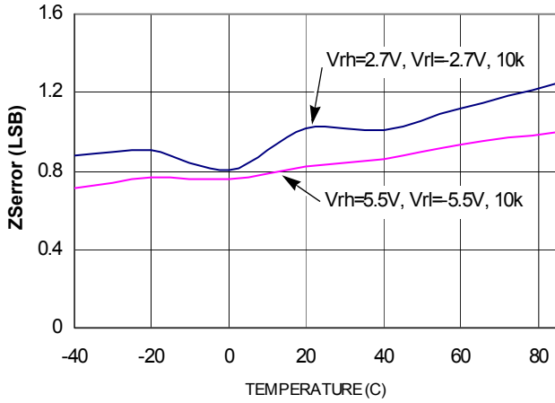
FIGURE 5. ZSensor vs TEMPERATURE
