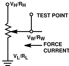
Test Circuit #2
