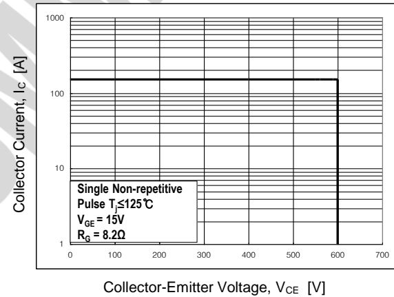
Fig 10. RBSOA Characteristic
