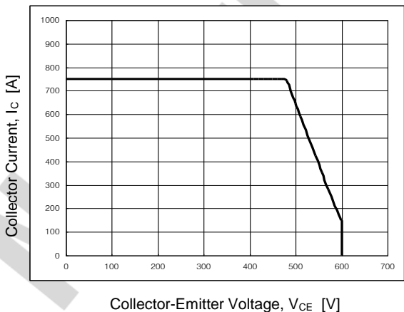
Fig 11. SCSOA Characteristic
