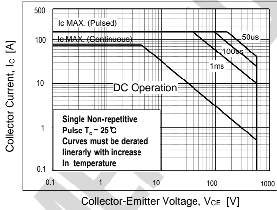
Fig14. SOA characteristics
