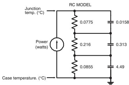
FIGURE 19b, TRANSIENT THERMAL IMPEDANCE MODEL
