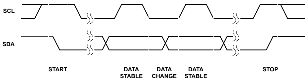
FIGURE 21. VALID DATA CHANGES, START, AND STOP CONDITIONS
