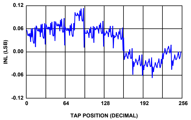
FIGURE 6. 50k \Omega INL vs TAP POSITION, V_{CC} = 3.3V , +25 °C
