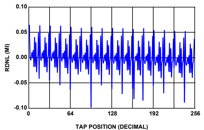
FIGURE 8. 50k \Omega RDNL vs TAP POSITION, V_{CC} = 3.3V , +25 °C
