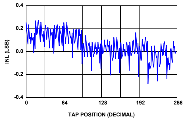
FIGURE 5. 10k \Omega INL vs TAP POSITION, V_{CC} = 3.3V , +25 °C
