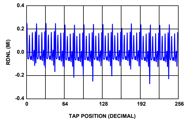
FIGURE 7. 10k \Omega RDNL vs TAP POSITION, V_{CC} = 3.3V , +25 °C
