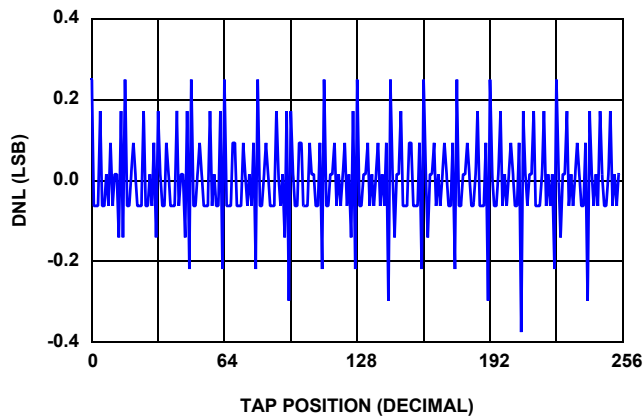
FIGURE 3. 10k \Omega DNL vs TAP POSITION, V_{CC} = 3.3V , +25 °C
