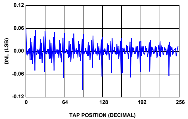
FIGURE 4. 50k \Omega DNL vs TAP POSITION, V_{CC} = 3.3V , +25 °C
