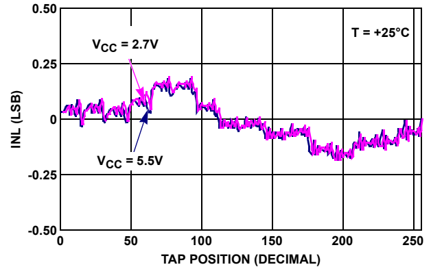
FIGURE 10. INL vs TAP POSITION IN RHEOSTAT MODE FOR 50kΩ (U)
