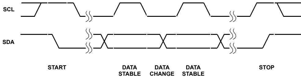
FIGURE 17. VALID DATA CHANGES, START, AND STOP CONDITIONS
