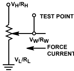
Test Circuit #2
