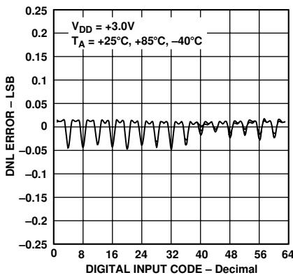
Figure 8. Potentiometer Divider Differential Nonlinearity Error vs. Code
