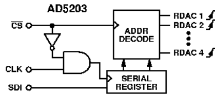
Figure 36. Equivalent Input Control Logic
