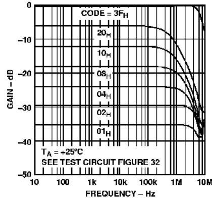
Figure 12. Gain vs. Frequency for R = 10\text{ k}\Omega
