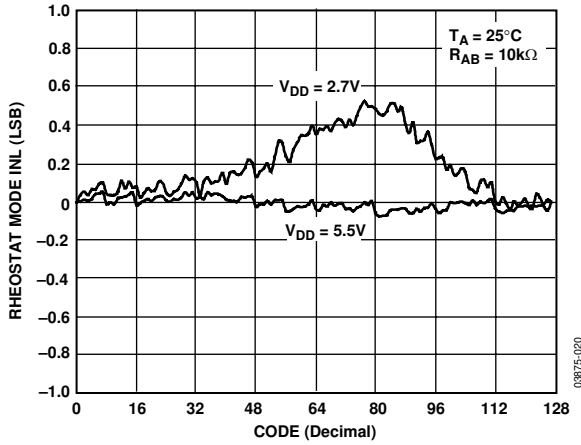
Figure 3. R-INL vs. Code vs. Supply Voltages
