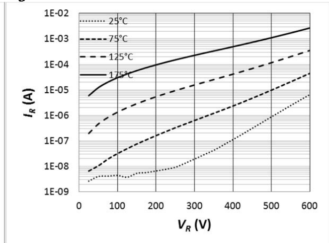
Fig. 18 Reverse Characteristics
