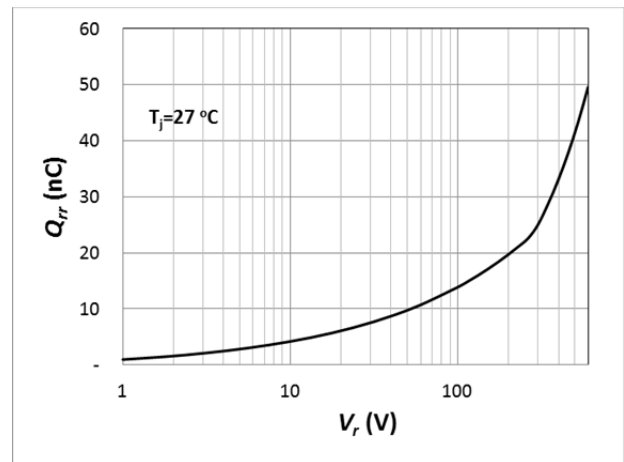
Fig. 22 Recovery Charge
