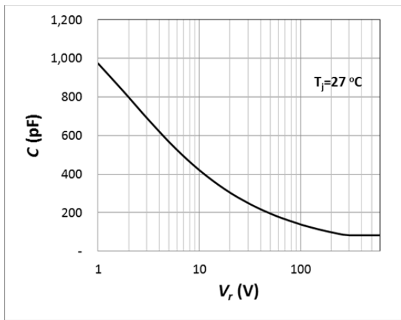
Fig. 21 Capacitance Curve
