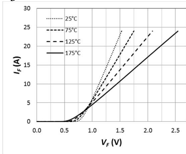
Fig. 17 Forward Characteristics
