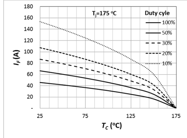
Fig. 20 Current Derating
