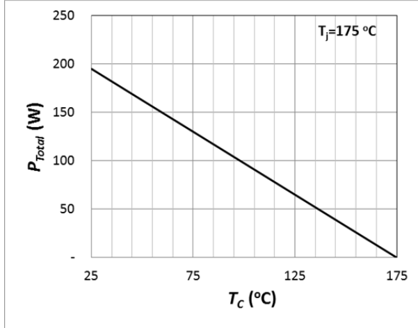
Fig. 19 Power Derating
