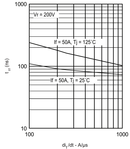
Fig. 9 - Typical Reverse Recovery Time vs. di_F/dt
