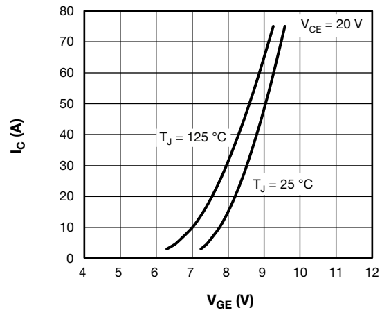
Fig. 4 - Typical Q1 - Q4 Trench IGBT Transfer Characteristics V CE = 20 V
