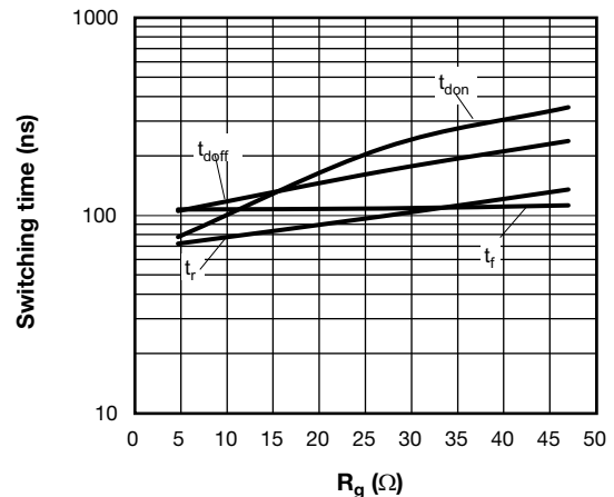
Fig. 10 - Typical Q1 - Q4 Trench IGBT Switching Time vs. R_g (with D5 - D6 Clamping Diode) T_J = 125\text{ }^\circ\text{C} , V_{CC} = 300\text{ V} , I_C = 75\text{ A} , V_{GE} = 15\text{ V} , L = 500\ \mu\text{H}
