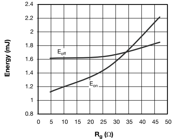
Fig. 9 - Typical Q1 - Q4 Trench IGBT Energy Loss vs. R_g (with D5 - D6 Clamping Diode) T_J = 125\text{ }^\circ\text{C} , V_{CC} = 300\text{ V} , I_C = 75\text{ A} , V_{GE} = 15\text{ V} , L = 500\ \mu\text{H}
