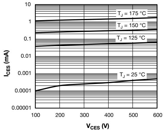
Fig. 24 - Typical Q2 - Q3 Trench IGBT Zero Gate Voltage Collector Current
