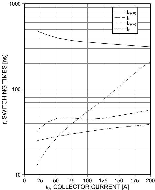
Figure 7. Typical switching times as a function of collector current (inductive load, T_j=175^\circ\text{C} , V_{CE}=400\text{V} , V_{GE}=15/0\text{V} , r_G=3,6\Omega , Dynamic test circuit in Figure E)
