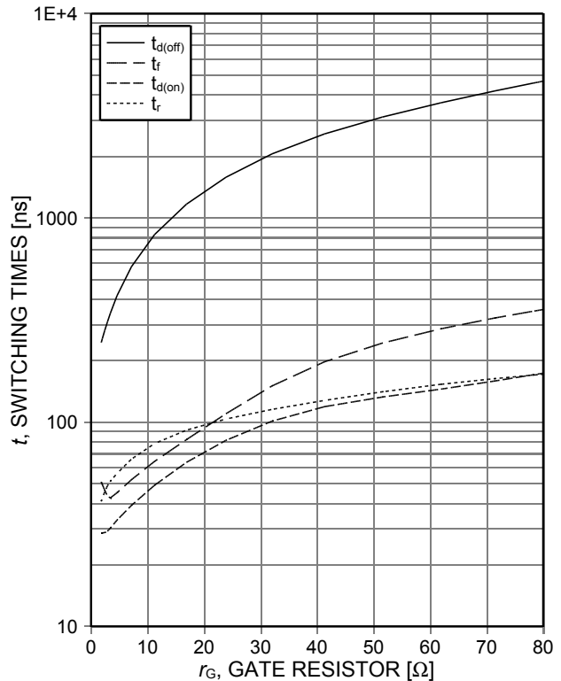
Figure 8. Typical switching times as a function of gate resistor (inductive load, T_j=175^\circ\text{C} , V_{CE}=400\text{V} , V_{GE}=15/0\text{V} , I_c=100\text{A} , Dynamic test circuit in Figure E)
