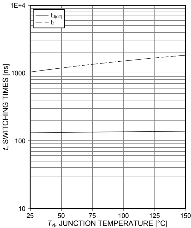
Figure 9. Typical switching times as a function of junction temperature (inductive load, V_{GE}=0/18V , I_C=15A , R_G=10.2\Omega , Dynamic test circuit in Figure E)
