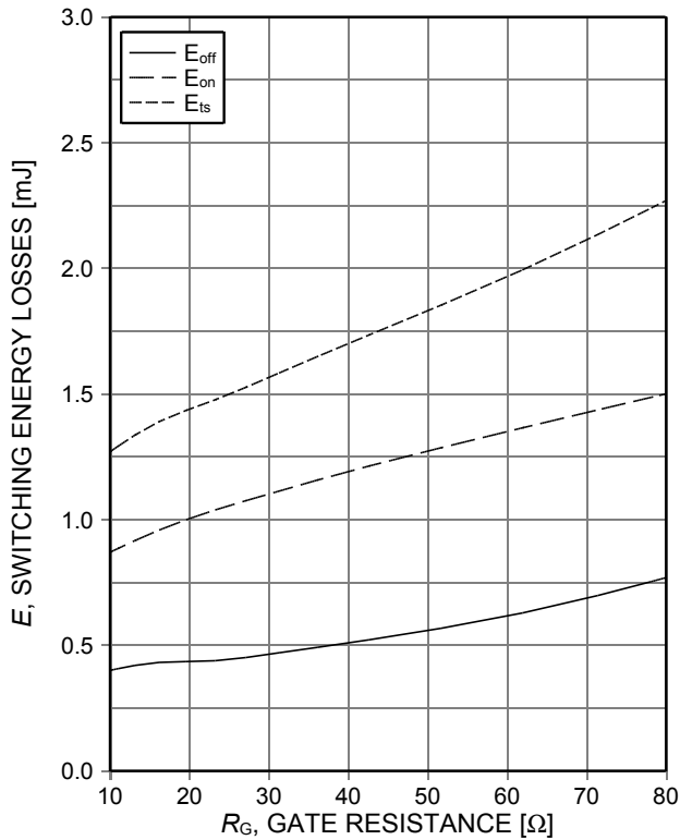
Figure 13. Typical switching energy losses as a function of gate resistance (inductive load, T_{vj}=175^\circ\text{C} , V_{CE}=400\text{V} , V_{GE}=0/15\text{V} , I_C=30\text{A} , dynamic test circuit in Figure E)
