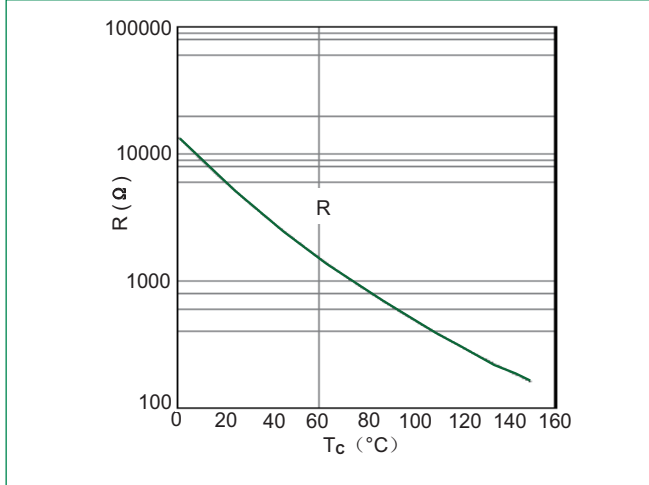
Figure 14: NTC Characteristics
