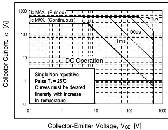
Fig 11. SOA Characteristic
