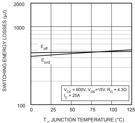
FIGURE 16, Energy Losses vs Junction Temperature
