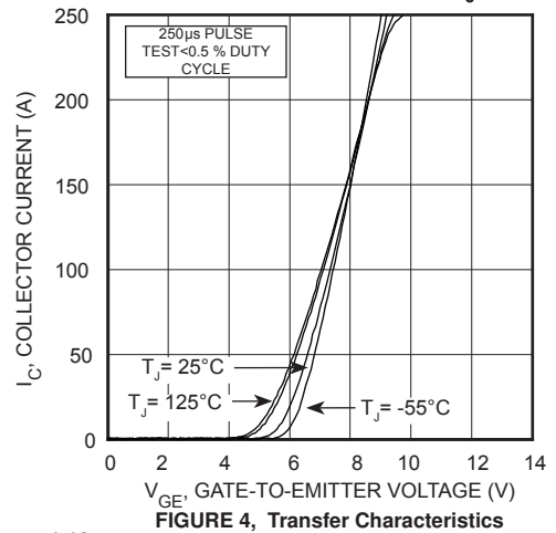
FIGURE 4, Transfer Characteristics
