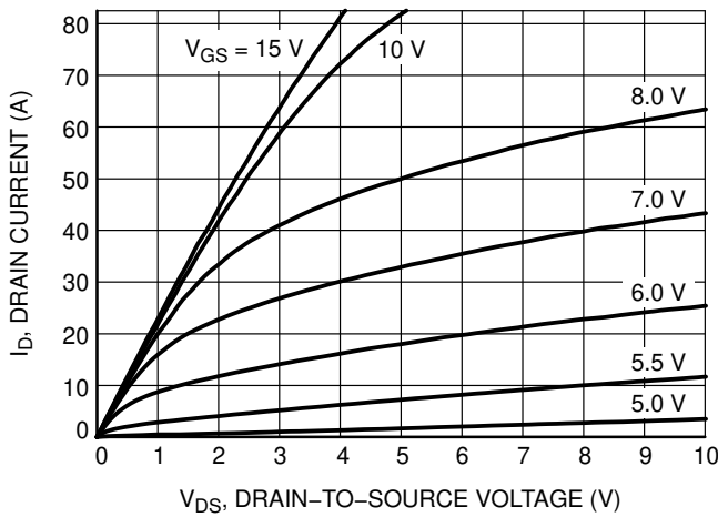
Figure 8. Saturation (25°C)
