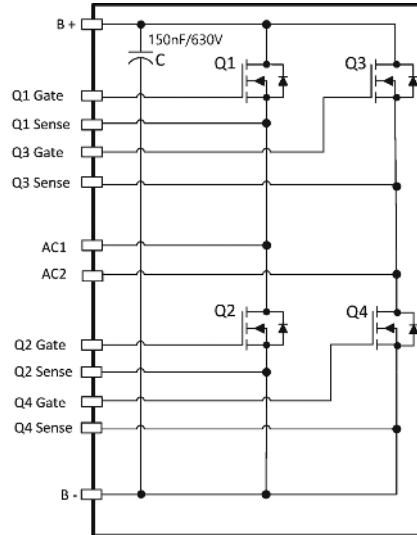
Figure 2. Schematic
