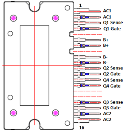
Figure 1. Pin Configuration
