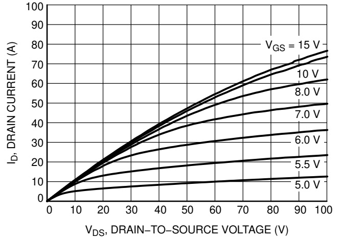
Figure 9. Saturation (150°C)
