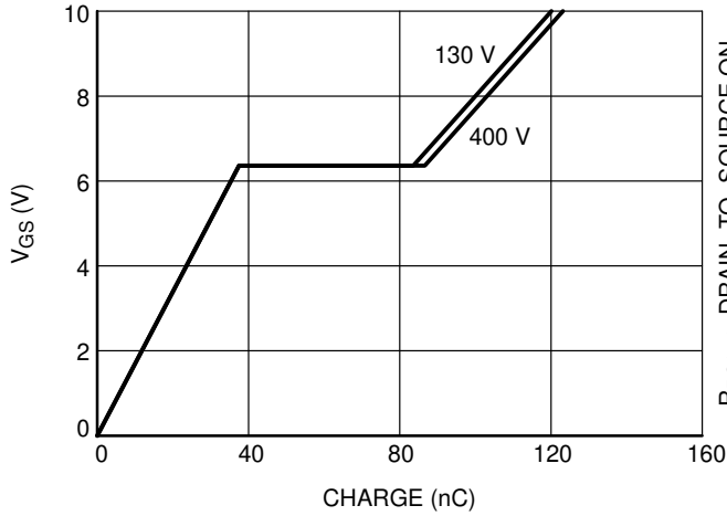
Figure 16. Gate Charge
