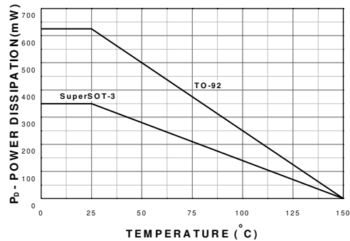
Figure 12. Power Dissipation vs Ambient Temperature
