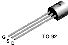
Figure 1. J111 / J112 / J113 Device Package
