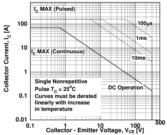
Figure 10. SOA Characteristics
