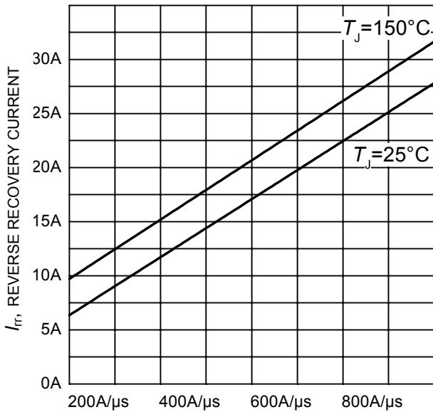
di_F/dt , DIODE CURRENT SLOPE
