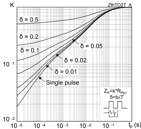
Figure 20. Thermal impedance
