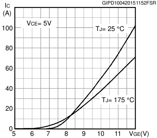
Figure 10: Transfer characteristics
