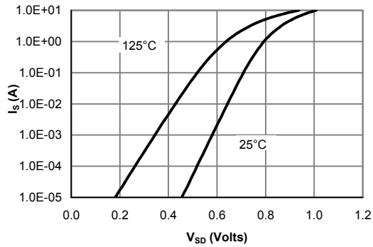
Figure 6: Body-Diode Characteristics
