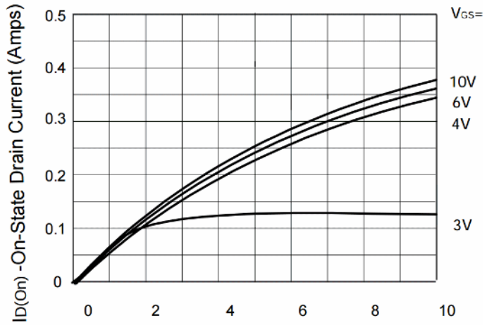
Saturation Characteristics
