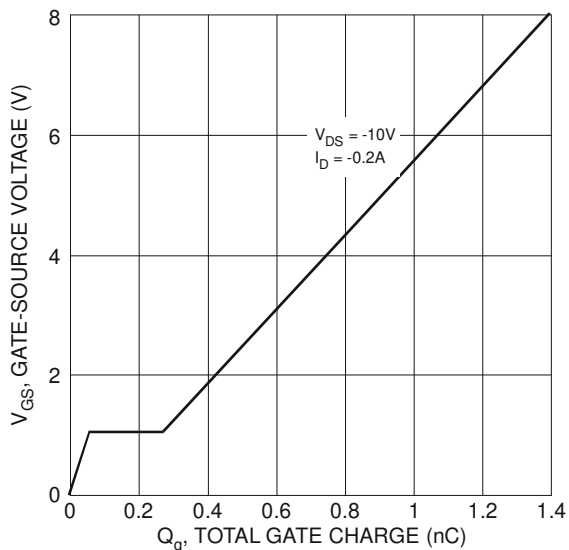
Figure 10 Gate-Charge Characteristics
