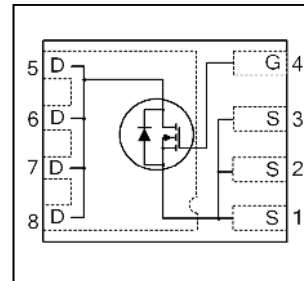
PQFN 3.3X3.3 mm
