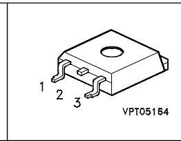
P-TO263-3-2
