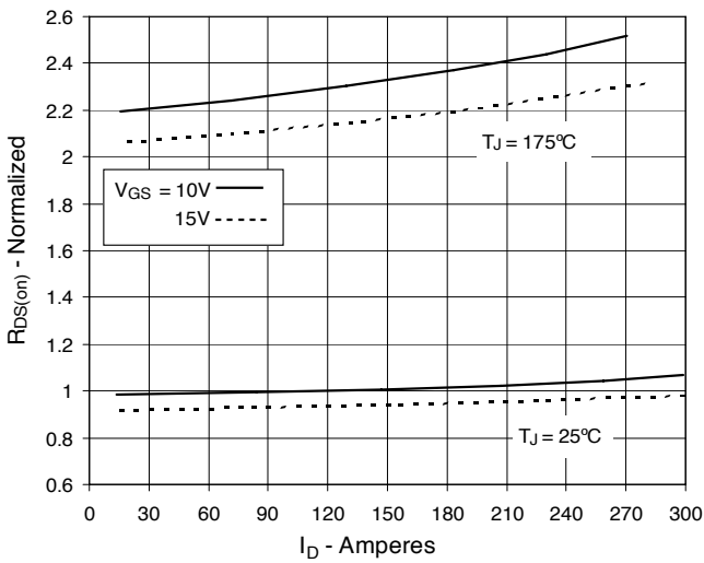
Fig. 5. R_{DS(on)} Normalized to I_D = 110A Value vs. Drain Current
