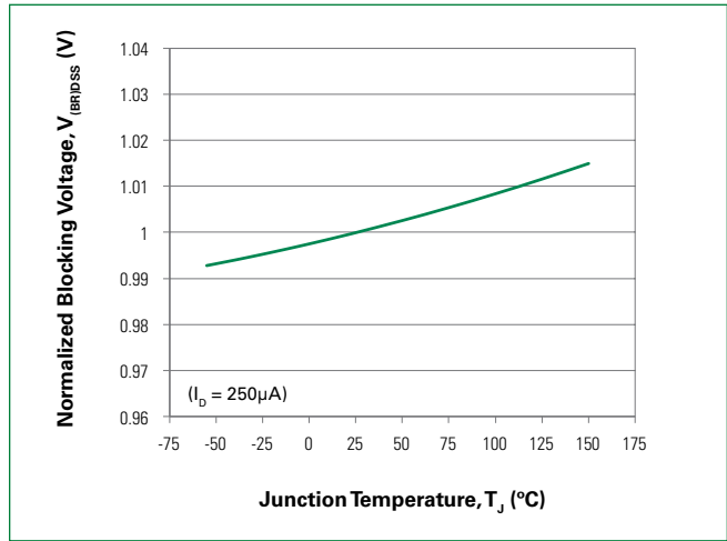
Figure 14: Drain-Source Blocking Voltage
