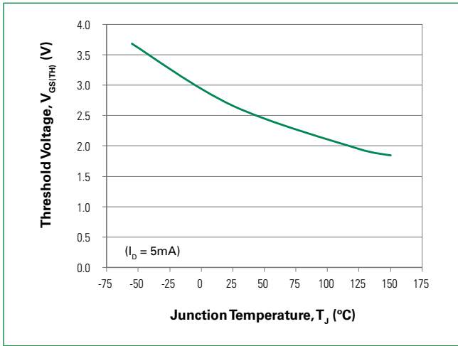
Figure 13: Threshold Voltage
