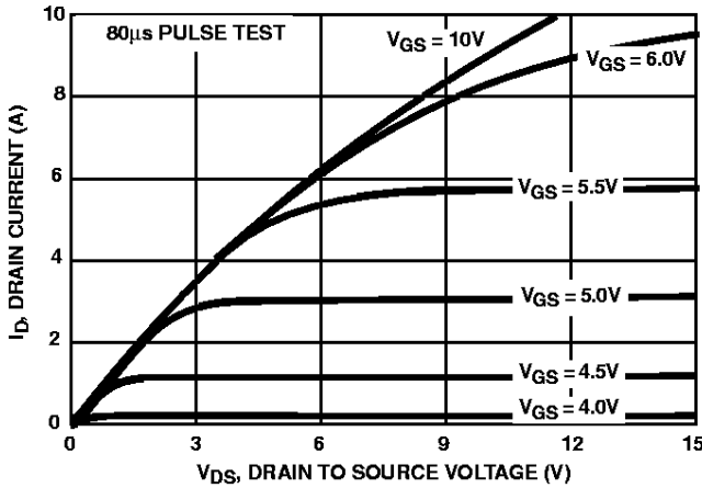
FIGURE 6. SATURATION CHARACTERISTICS
