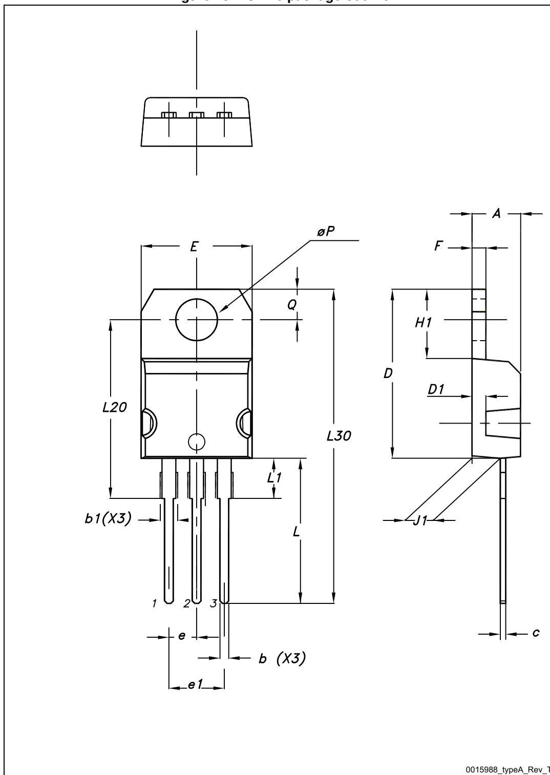
Figure 28. TO-220 package outline
