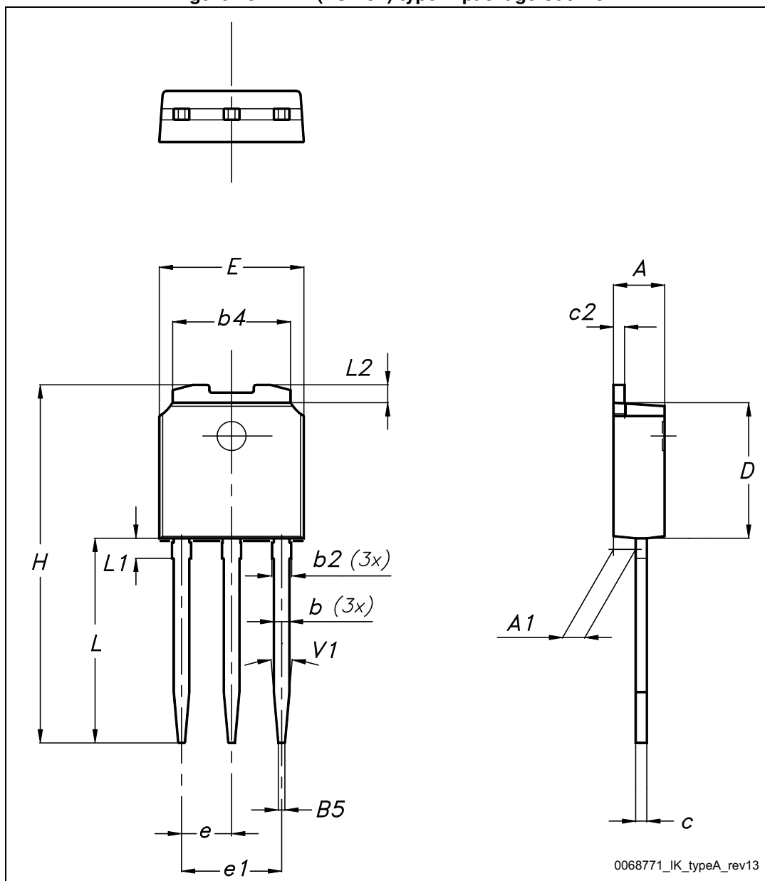
Figure 29. IPAK (TO-251) type A package outline
